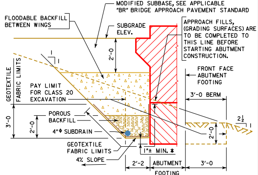
SECTION A-A BACKFILL DETAILS
