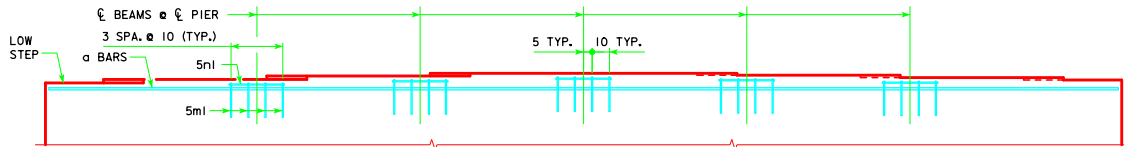
PART ELEVATION VIEW OF PIER CAP
