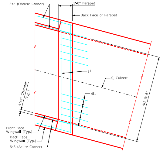
Detail A (Showing parapet bars only)
