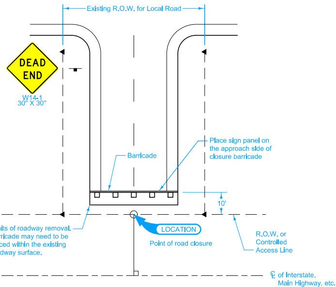
PLAN - INSTALLATION
