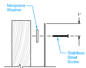
SIGN PANEL INSTALLATION
