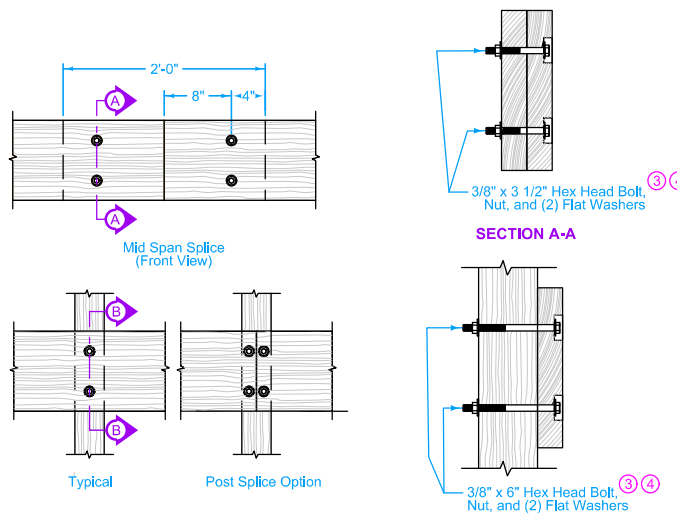
WOOD FRAME ASSEMBLY
