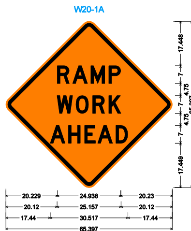
W20-1A; 48,000" across sides 3.000" Radius, 1.250" Border, 0.750" Indent, Black on Orange; [RAMP] D; [WORK] D; [AHEAD] D;
