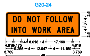
G20-24; 1.500" Radius, 0.625" Border, 0.375" Indent, Black on Orange; [DO NOT FOLLOW] C; [INTO WORK AREA] C;
