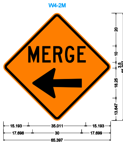
W4-2M; 48,000" across sides 3.000" Radius, 1.250" Border, 0.750" Indent, Black on Orange; [MERGE] C; Arrow K-30, 180°;
