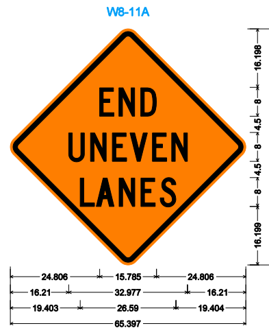
W8-11A; 48,000" across sides 3.000" Radius, 1.250" Border, 0.750" Indent, Black on Orange; [END] C; [UNEVEN] C; [LANES] C;
