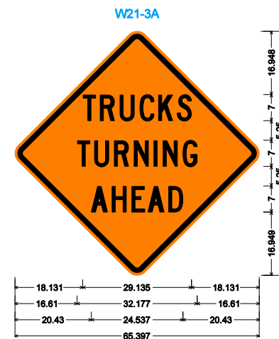
W21-3A; 48,000" across sides 3.000" Radius, 1.250" Border, 0.750" Indent, Black on Orange; [TRUCKS] C; [TURNING] C; [AHEAD] C;
