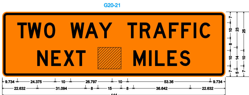
G20-21; 3.000" Radius, 1.250" Border, 0.750" Indent, Black on Orange; [TWO WAY TRAFFIC] D; [NEXT] D; Rectangle Orange; [MILES] D;
