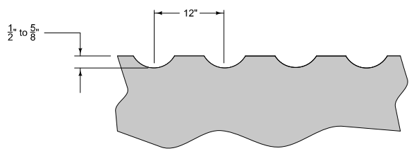
SECTION
