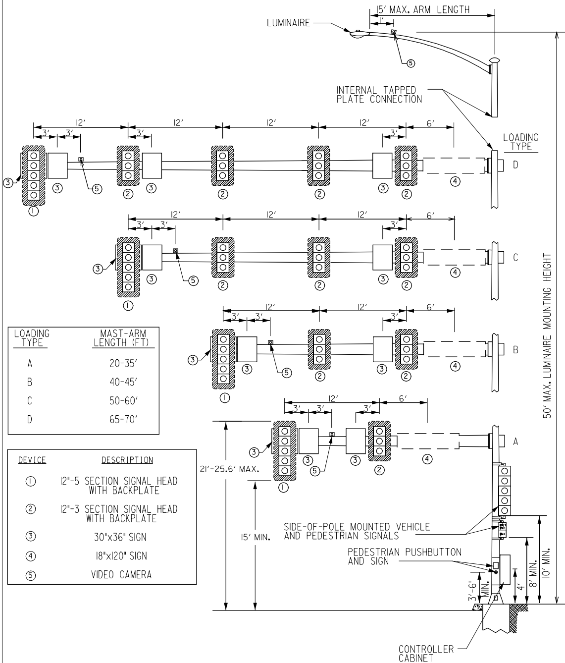
MAST ARM POLE LOADING
