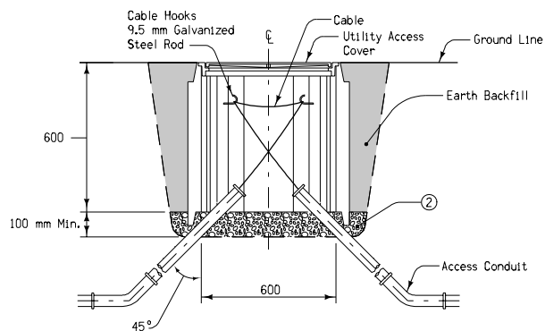
TYPE 1 SECTION A-A
