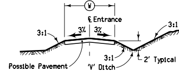
ENTRANCE TYPICAL SECTION
