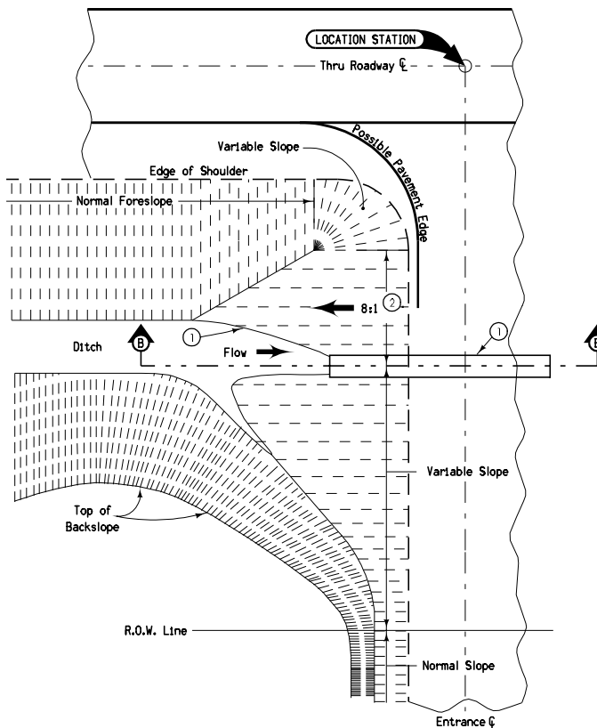
TYPE B OR C ENTRANCE WITH PIPE
