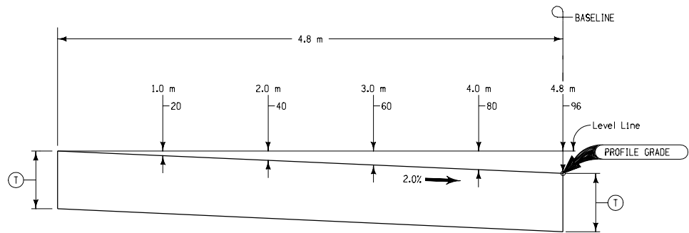
CROSS SECTION
