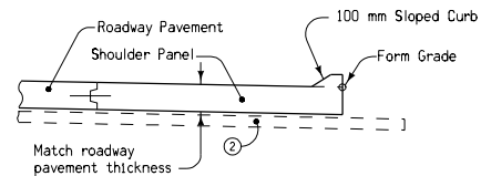
SECTION A-A (Shoulder Panel)
