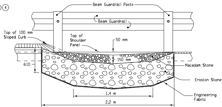
SECTION C-C
