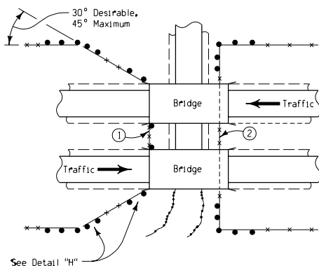
TYPICAL DETAILS FENCING AT DUAL BRIDGES OVER STREAM AND SIDE ROAD
