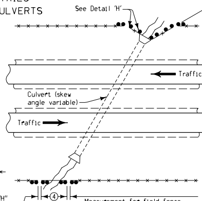
TYPICAL DETAILS FENCING AT CULVERTS
