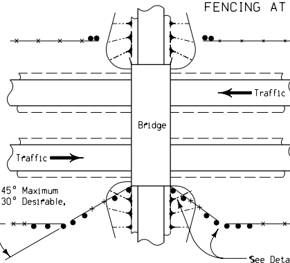
TYPICAL DETAILS FENCING AT BRIDGE FOR SIDE ROAD OVER
