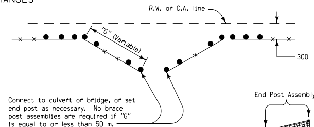
DETAIL 'H'
