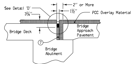
DETAIL 'E'
