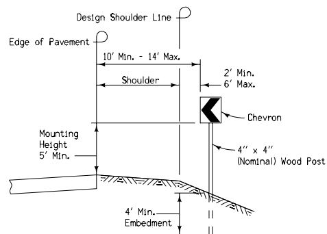
TYPICAL SECTION
