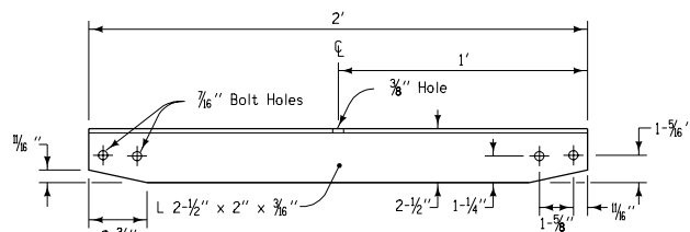
BRACE DETAIL
