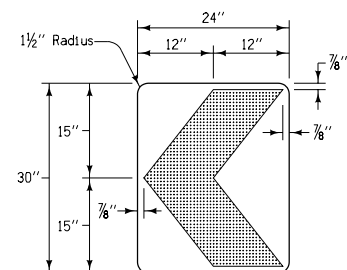
CHEVRON ALIGNMENT SIGN (W1-8)
