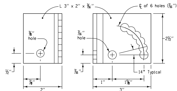
BRACKET DETAIL
