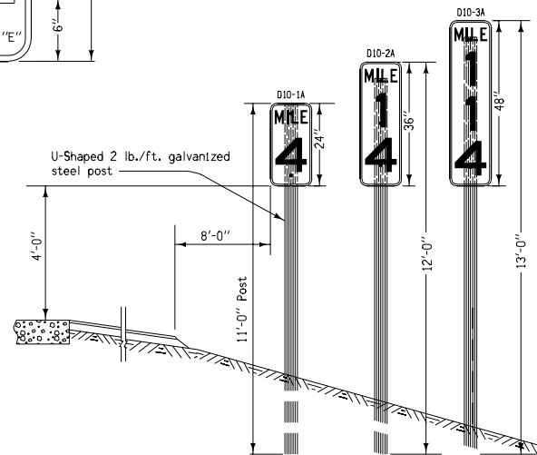
MILEPOST MARKER - SHOULDER ERECTION
