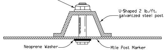
TOP VIEW MILEPOST MARKER ASSEMBLY
