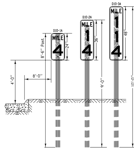
MILEPOST MARKER - CURB ERECTION
