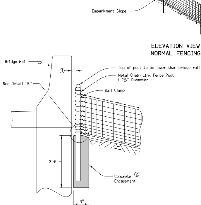
PARTIAL ELEVATION VIEW DETAIL "A"
