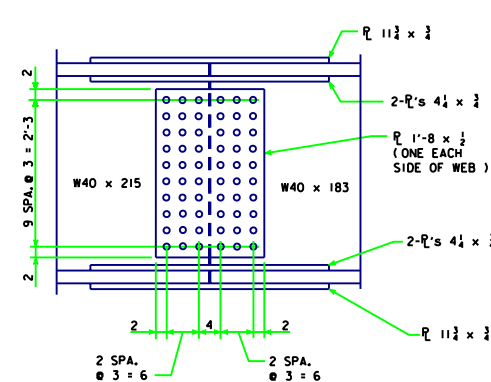
TOP AND BOTTOM FLANGE
