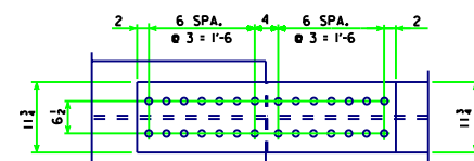
TOP AND BOTTOM FLANGE
