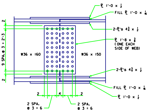
BOLTED SPLICE DETAILS
