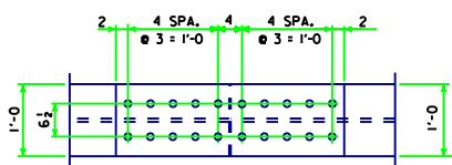
TOP AND BOTTOM FLANGE
