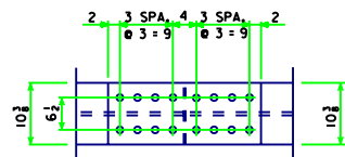
TOP AND BOTTOM FLANGE
