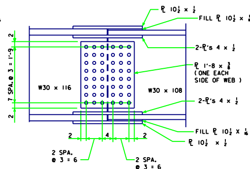
BOLTED SPLICE DETAILS
