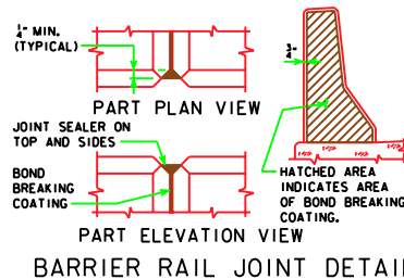
BARRIER RAIL JOINT DETAILS
