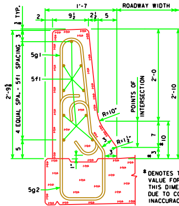
PART SECTION A-A
