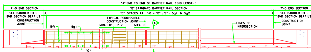
ELEVATION OF BARRIER RAIL
