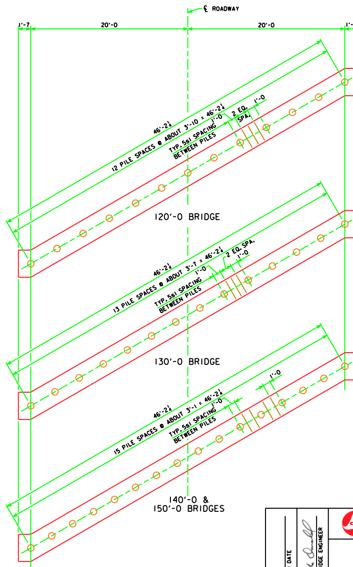
PILE PLAN - 30° SKEW WOOD PILING
