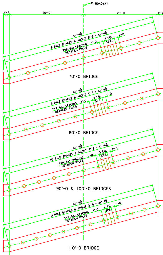
PILE PLAN - 15° SKEW WOOD PILING
