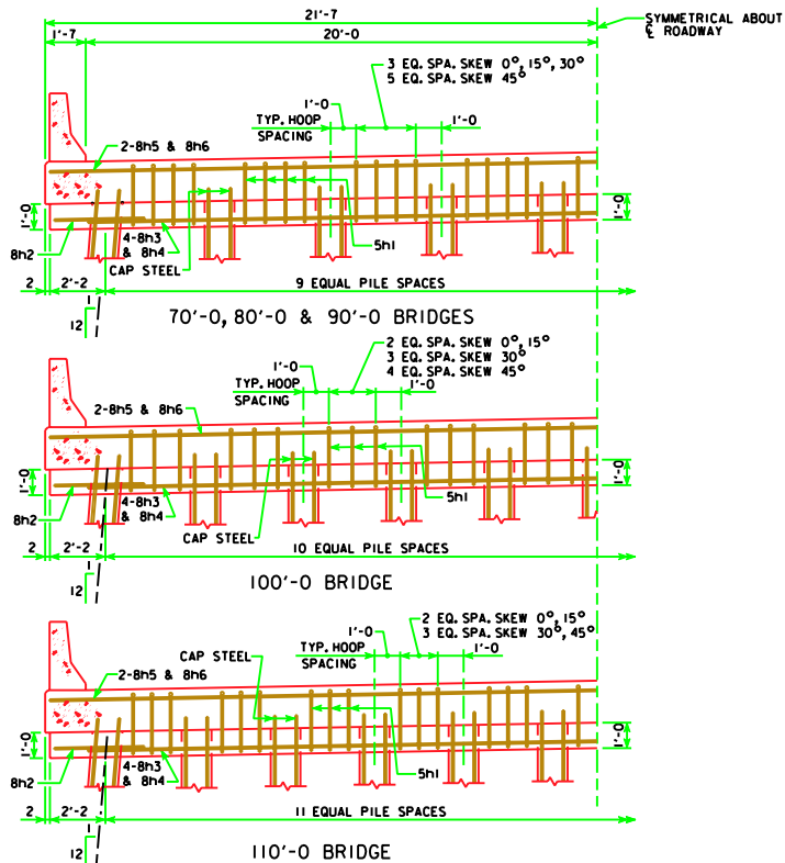
HALF SECTION NEAR PIER SHOWING STIRRUP SPACING AND NUMBER OF PILING NOTE: BOTTOM OF CAP ELEVATIONS WILL BE REQUIRED AT THE OF ROADWAY AND AT EACH EXTERIOR PILE.
