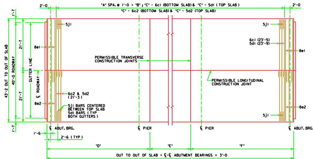
0° SKEW TRANSVERSE REINFORCING STEEL LAYOUT
