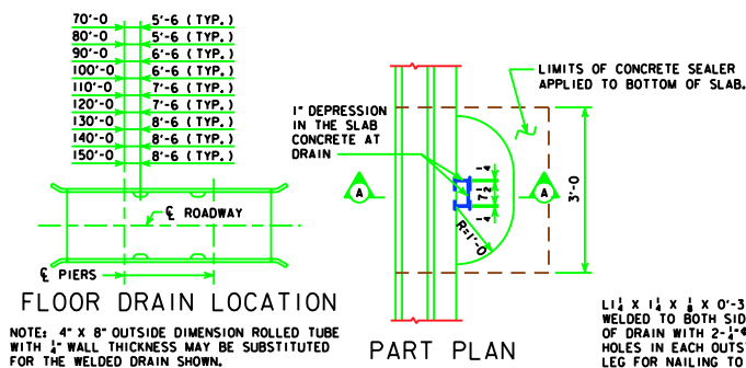
FLOOR DRAIN DETAILS
