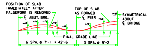
THIS DIAGRAM SHOWS THE FORM CAMBER REQUIRED TO COMPENSATE FOR THE ANTICIPATED ULTIMATE DEAD LOAD DEFLECTION. THE ABOVE DIMENSIONS DO NOT INCLUDE ANY ALLOWANCE FOR FORM DEFLECTION OR FALSEWORK SETTLEMENT.
