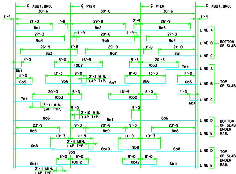
PLACEMENT FOR LONGITUDINAL REINFORCEMENT
