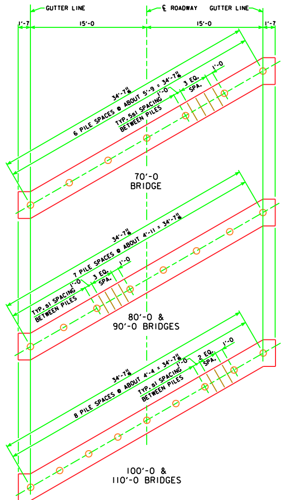
PILE PLAN - 30° SKEW WOOD PILING
