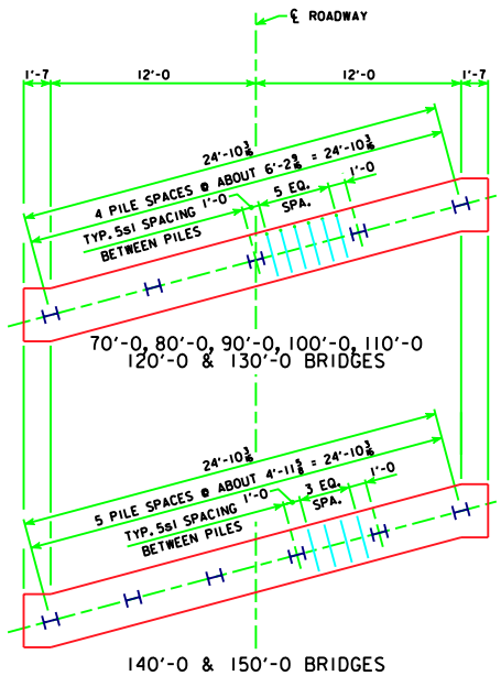
PILE PLAN - 15° SKEW STEEL PILING
