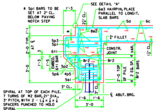
SECTION NORMAL TO ABUTMENT AT RAIL
