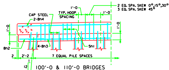
100'-0 & 110'-0 BRIDGES
