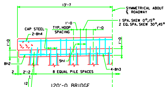
120'-0 BRIDGE
