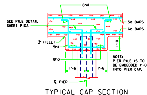
TYPICAL CAP SECTION
