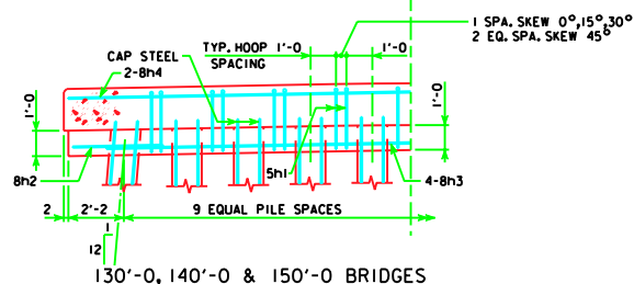
130'-0, 140'-0 & 150'-0 BRIDGES
