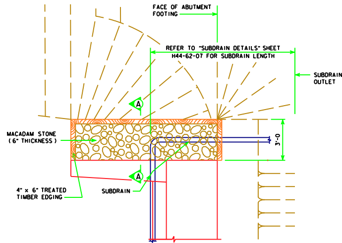
TOP VIEW OF WING ARMORING
