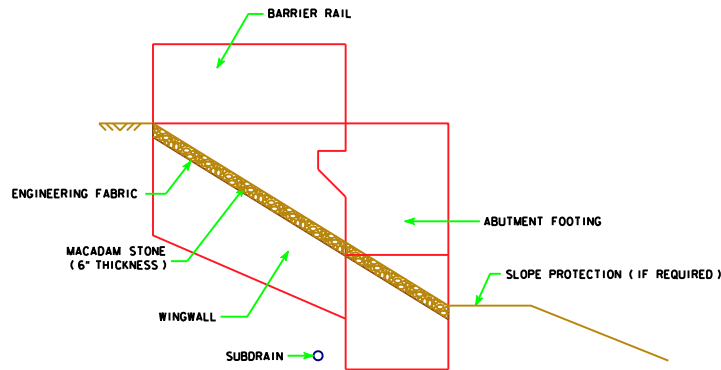
PROFILE VIEW OF WING ARMORING
