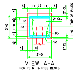
VIEW A-A FOR 9, 10, 11, 12, 13 & 14 PILE BENTS
