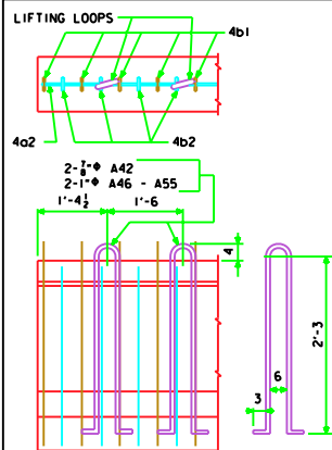
LIFTING LOOP DETAIL
