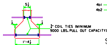
COIL TIE DETAIL
