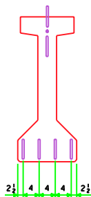
STRAND PROJECTION AT BEAM ENDS WHEN EMBEDDED IN CONCRETE END DIAPHRAGMS
