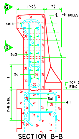
SECTION B-B
