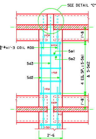
PART SECTION AT PIER
