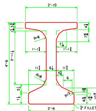
BTD BEAM CROSS SECTION
