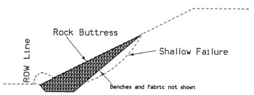
Figure 8: Slope repair with rock buttress (from Lohnes, et.al., 2001).
