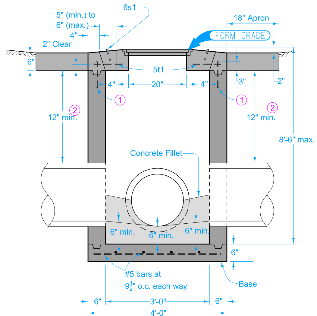
TYPICAL SECTION
