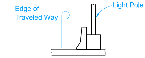
TYPE 5 Concrete Barrier Rail or Bridge Rail
