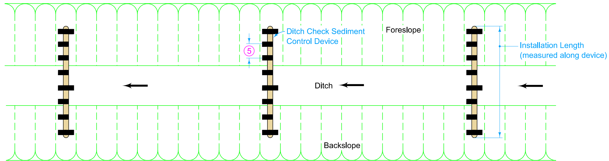
DITCH PROTECTION 6
