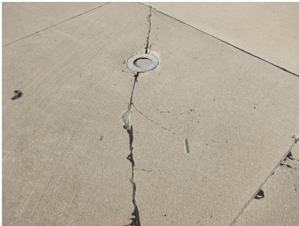
T02PO-02. LTD Cracking (Sample Unit No. 03).
