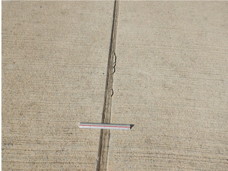
A02IC-02. Joint Seal Damage (Sample Unit No. 08).
