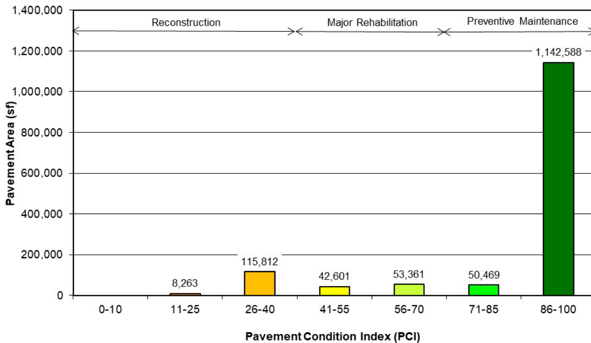
Figure 6. Pavement area by PCI range at Iowa City Municipal Airport.
