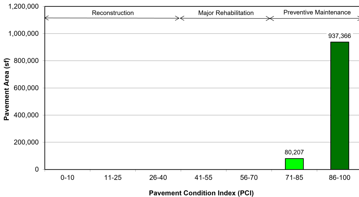
Figure 6. Pavement area by PCI range at James H Connell Field at Independence Municipal Airport.
