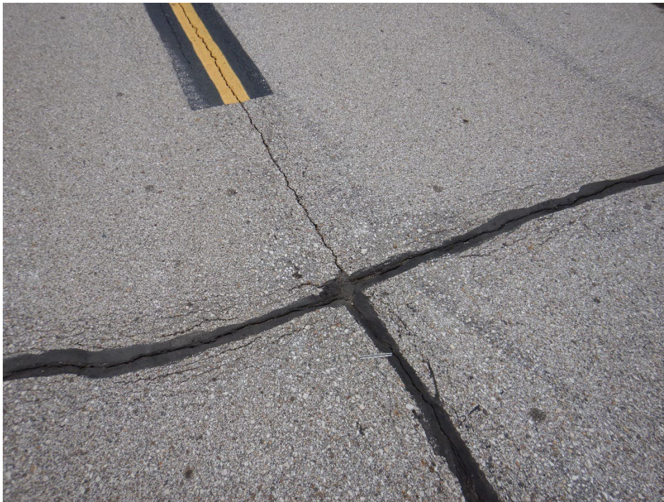
T01HU-01. L&T Cracking (Sample Unit No. 01).
