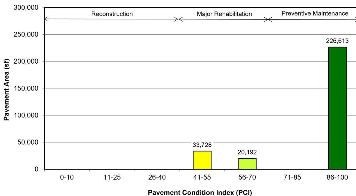
Figure 6. Pavement area by PCI range at Humboldt Municipal Airport.
