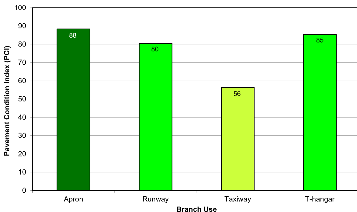
Figure 7. Area-weighted PCI by branch use at Forest City Municipal Airport/Trimble Field. (Values on chart are area weighted.)
