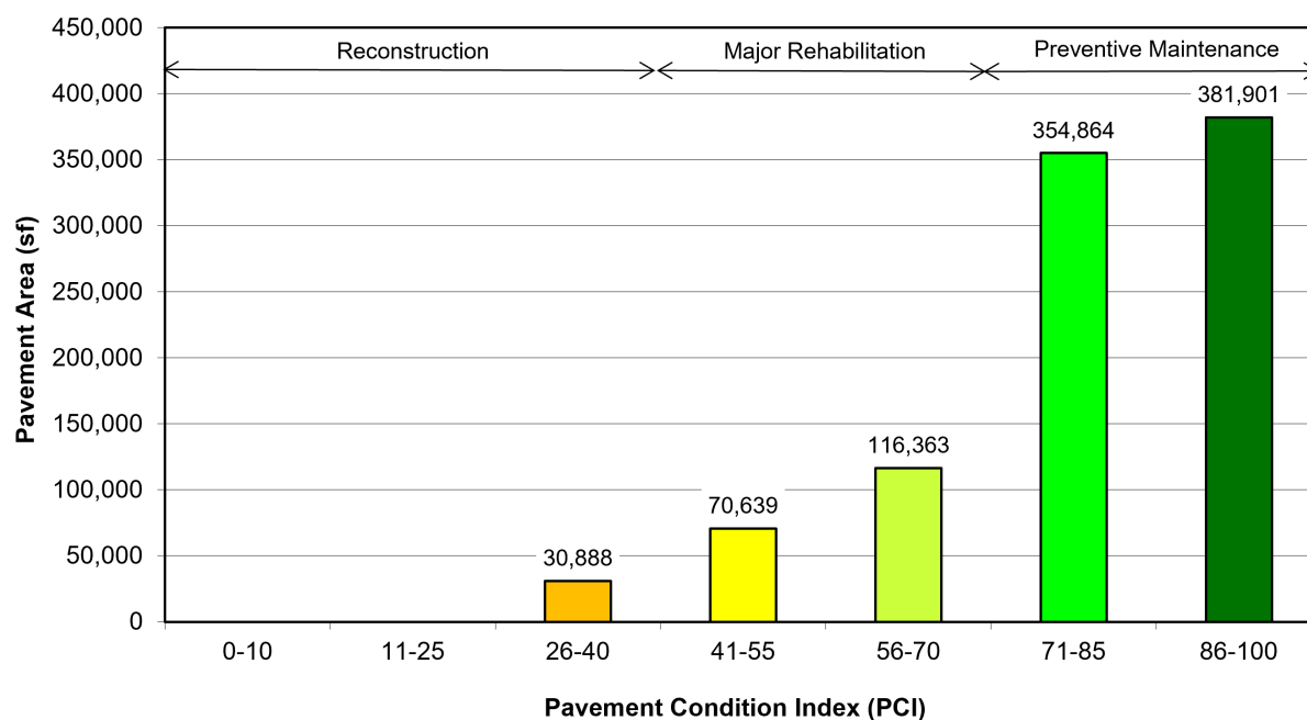
Figure 6. Pavement area by PCI range at Forest City Municipal Airport/Trimble Field.
