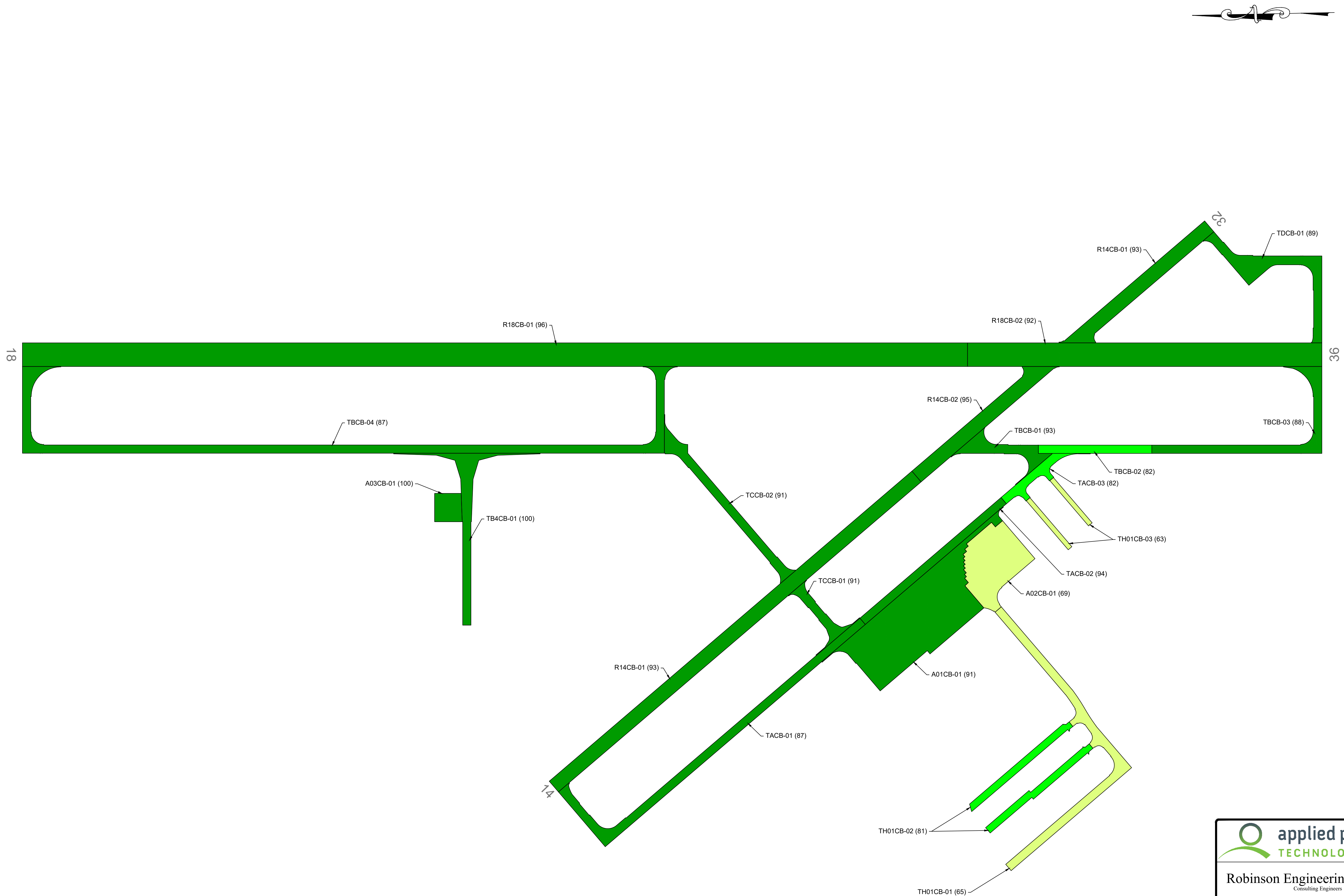
FIGURE 8. PCI MAP.
