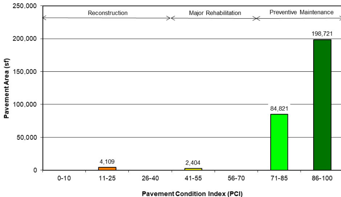
Figure 6. Pavement area by PCI range at Bloomfield Municipal Airport.
