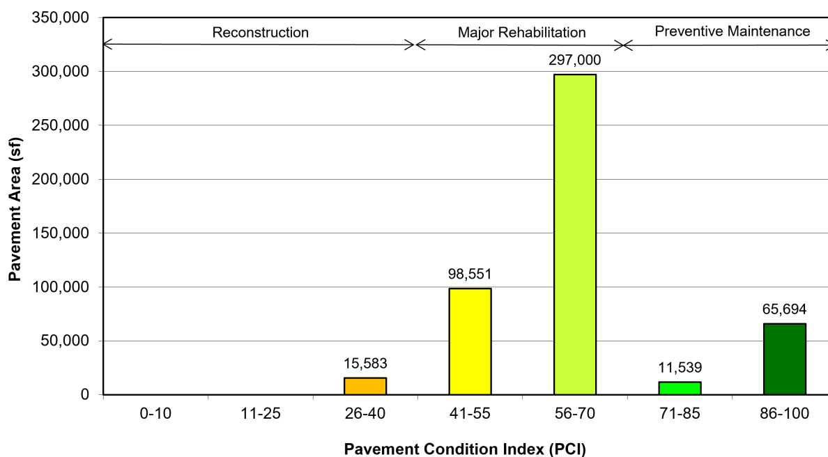
Figure 6. Pavement area by PCI range at Algona Municipal Airport.
