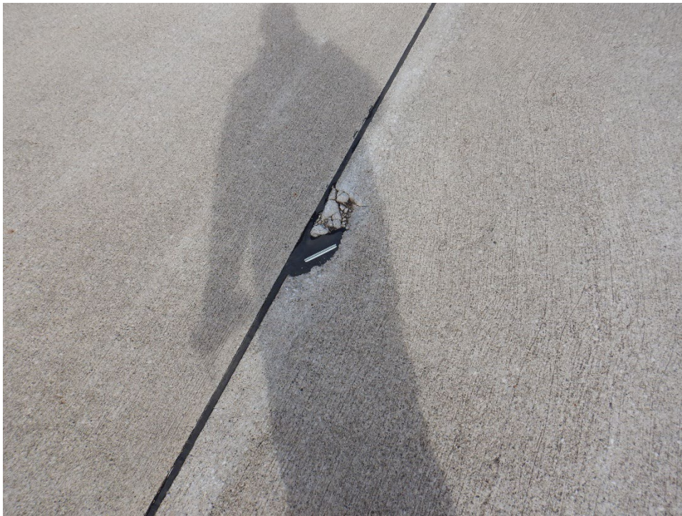
A01AG-01. Joint Spalling (Sample Unit No. 06).
