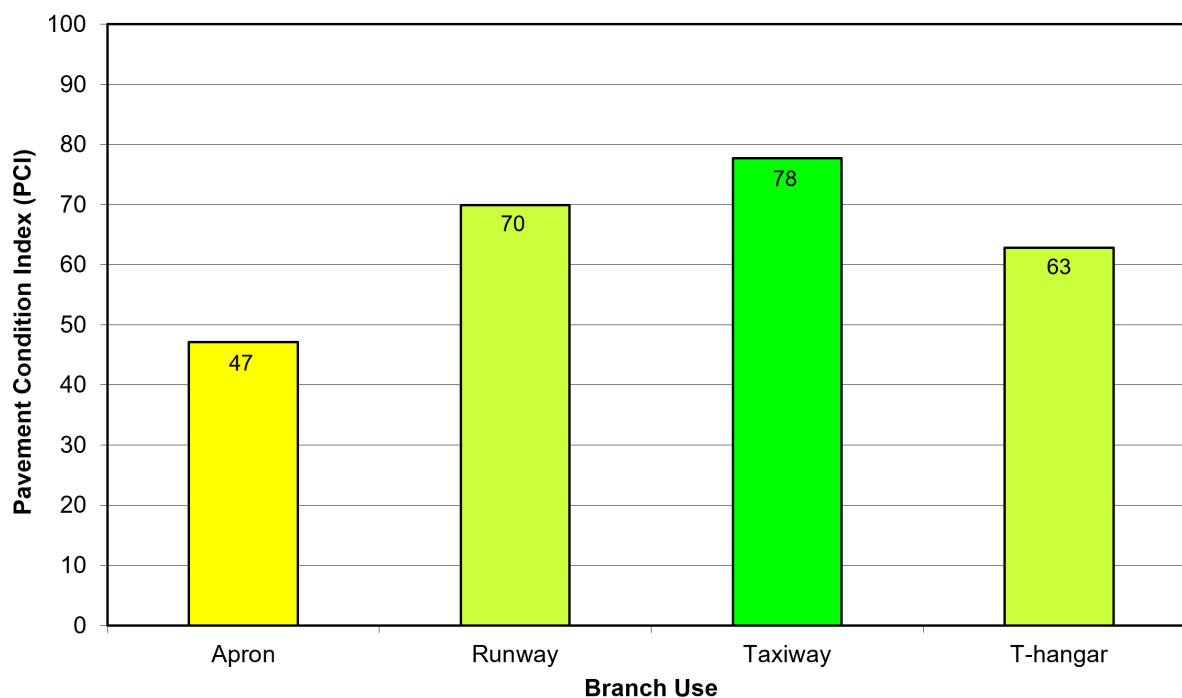
Figure 7. Area-weighted PCI by branch use at Algona Municipal Airport. (Values on chart are area weighted.)
