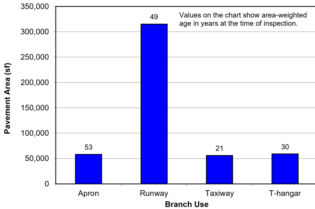
Figure 2. Pavement area by branch use at Algona Municipal Airport.
