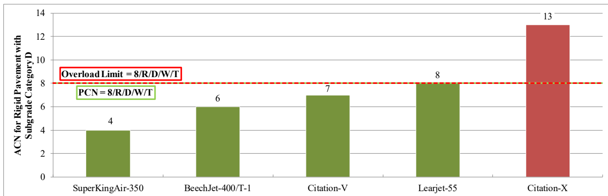
Figure 1. ACN–PCN comparison for Runway 4/22.
